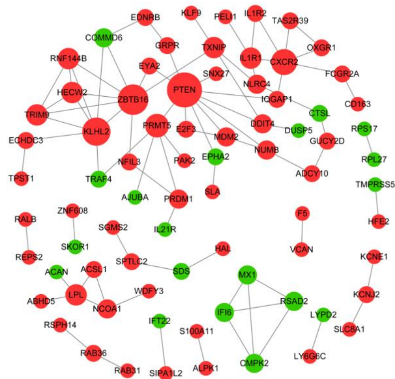
Figure 3: Protein-protein interaction network. Nodes in red circle indicate up-regulated DEGs, while node in green circle indicates down-regulated DEGs. Node size is proportional to its degree value.
