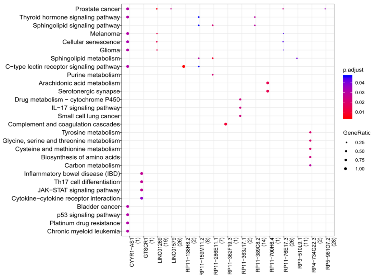
Figure 4: Results of pathway prediction for LncRNA. The color changes from red to blue represent the p values from small to large, while the bubble size indicates the proportion of gene counts involved in one term to all genes.
